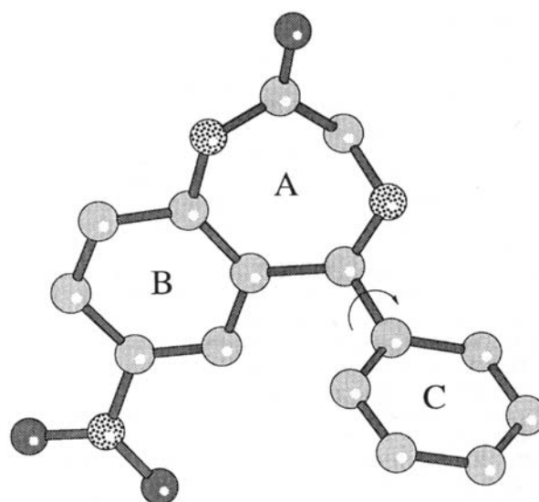
Fig. 6. Crystal structure of nitrazepam, a benzodiazepine derivative [33]. In solution, ring C may rotate with reference to the diazepam ring A.
