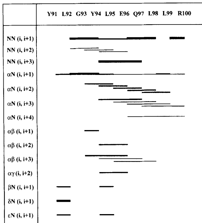
Fig. 3. Summary of the ^1H/^1H NOE connectivities for the decapeptide in SDS/water. The intensity of the NOE cross-peaks is indicated by the thickness of the lines, classified as strong, medium and weak.
