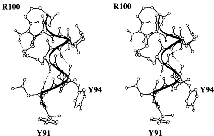
Fig. 5. Stereoviews of the decapeptide time-averaged structure from the last 30 ps of restrained-MD simulation.
