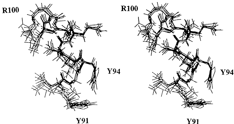
Fig. 4. Ten superimposed structures of the decapeptide, extracted from the last 30 ps of restrained-MD simulation.
