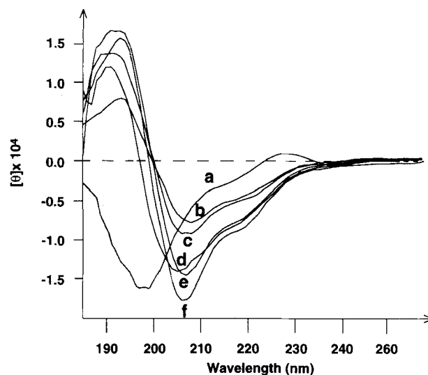
Fig. 1. CD spectrum of the benzodiazepine-like decapeptide in water as a function of SDS concentration. The peptide concentration was 79 μM. The SDS concentration was (a) 0.0, (b) 1.5, (c) 3 (d) 15, (e) 30 and (f) 200 mM.
