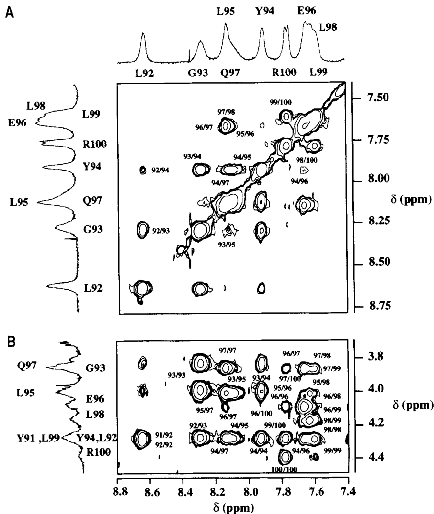
Fig. 2. Portion of the decapeptide NOESY spectrum in SDS/water showing the NH/NH (A) and C\alpha H/NH (B) NOE connectivities. Peptide concentration, 5 mM; SDS concentration, 0.20 M; \tau_m = 200 ms.
